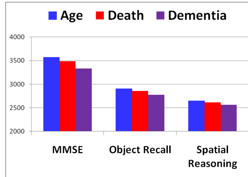
ML BIC
